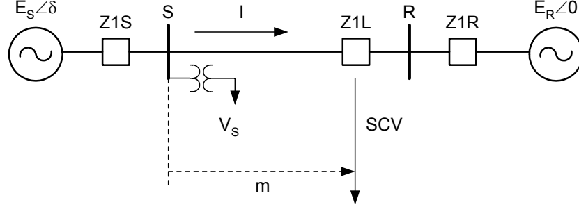
Figure 29 A Two-Source Power System
