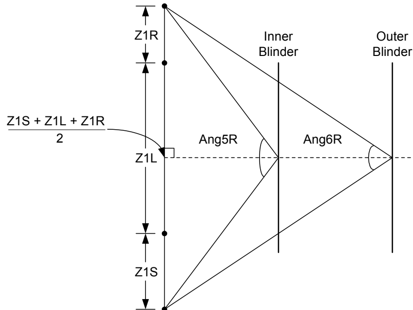
Figure 3 Equivalent Two-Source Machine Angles During OOS
