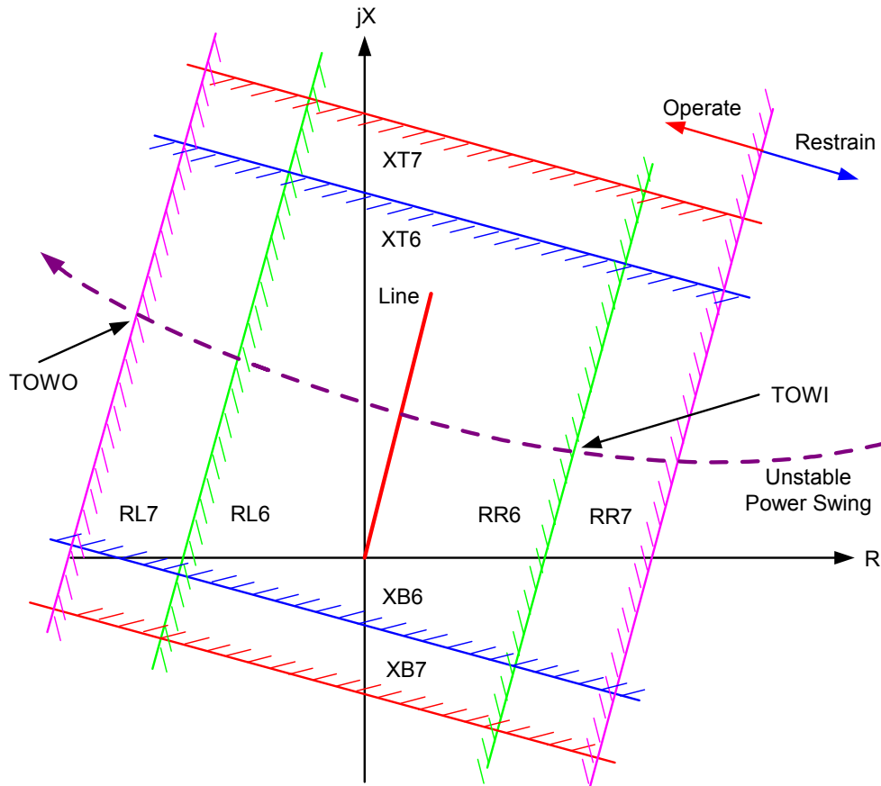
Figure 21 OST Scheme Blinder Characteristics
