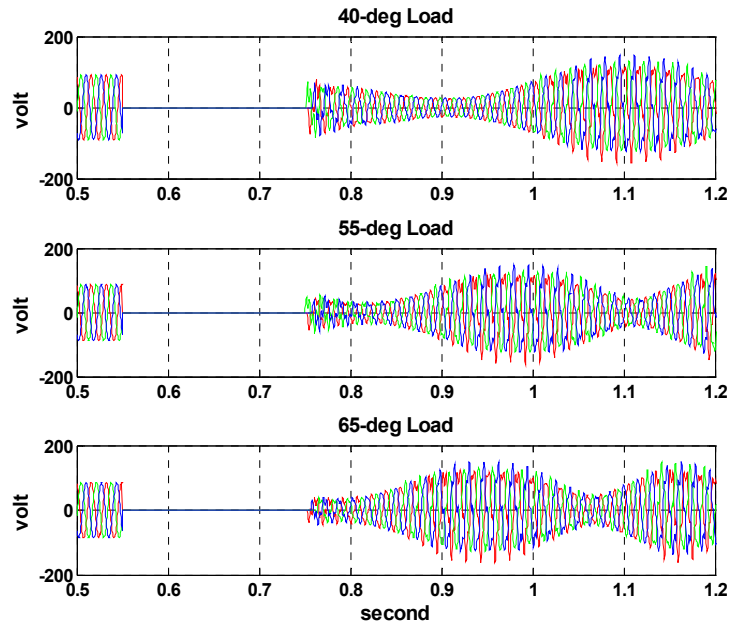
Figure 26 Voltages of Example 2 With Different Loads
