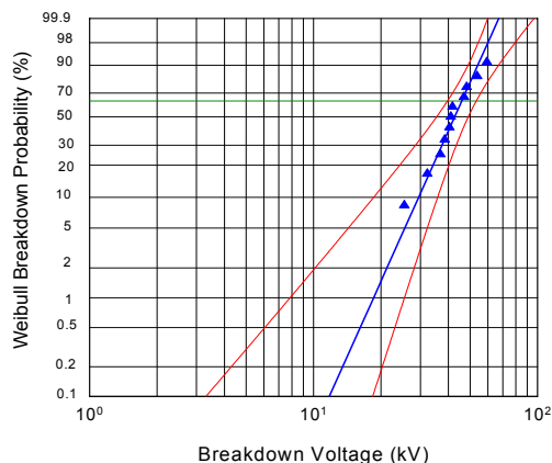
Fig. 1. Weibull distribution of 60 Hz breakdown voltages 11 cables \alpha = 45.9 kV peak \beta = 5.08 Confidence Intervals 95%
