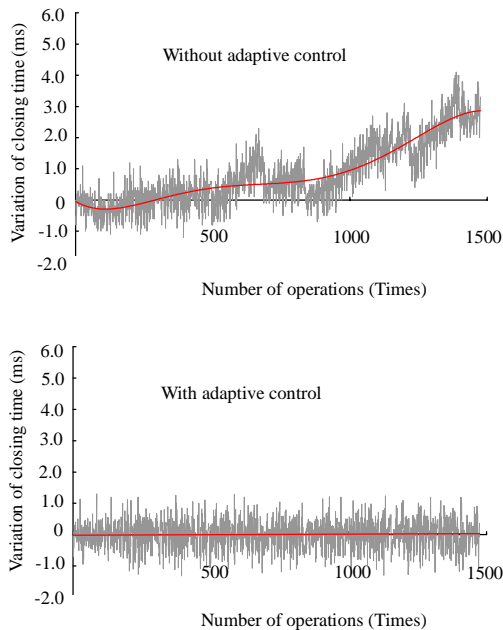
Fig.10 Typical drifts of the closing times measured with adaptive control of controller and without adaptive control
