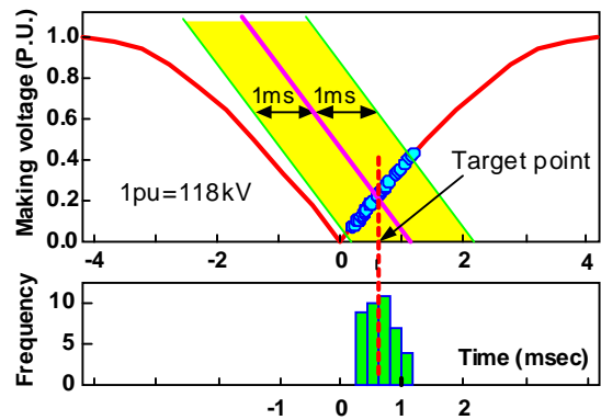
Fig.11 (a) Distribution of making voltages and closing instants using a 145kV GCB
