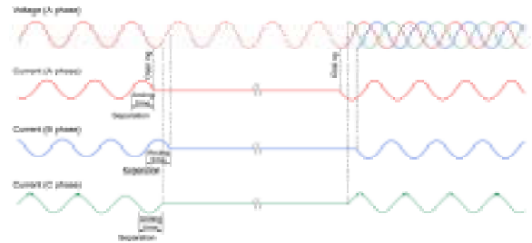
Fig.14 Voltage and current behavior of controlled shunt reactor de-energization and energization
