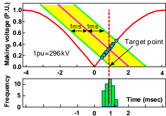
Fig.11 (b) Distribution of making voltages and closing instants using a 362kV GCB
