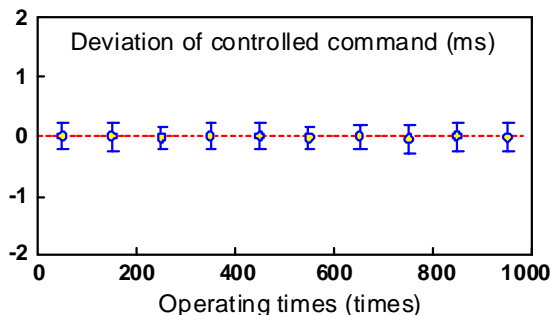
Fig.9 Deviation of the controlled switching commands issued by the controller during the consecutive operations
