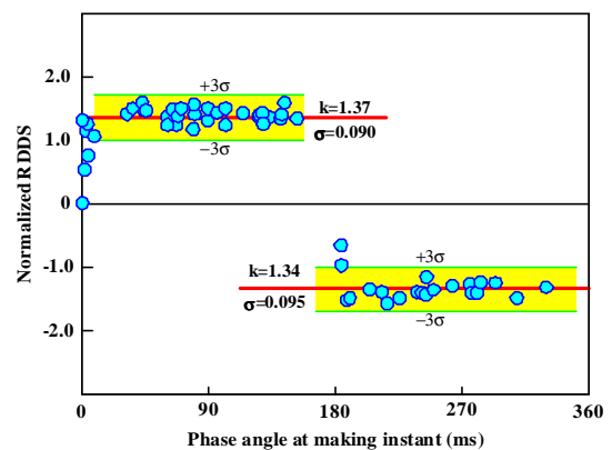
Fig.4 RDDS measurement obtained by pre-strike test
