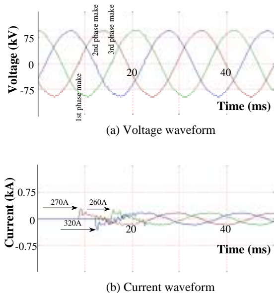
Fig.12 (b) Waveforms of the 10 th capacitor energization
