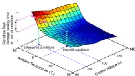
Fig.2 Deviation from the average closing time at the standard conditions plotted as functions of the ambient temperature and the control voltage.
