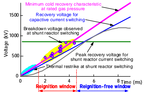
Fig.7 Dielectric recovery (RRDS) characteristic of the 550kV one-break GCB
