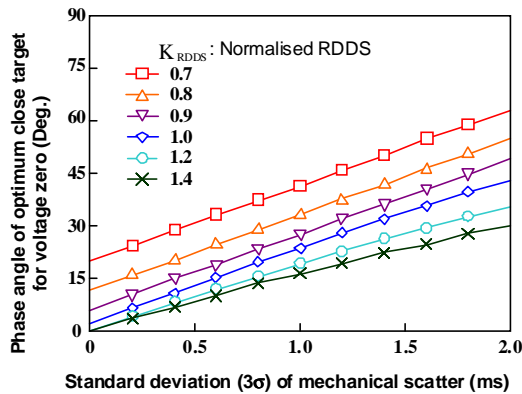
Fig.5 Optimum close target for voltage zero calculated as functions of RDDS and Mechanical scatters
