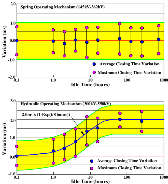
Fig.8 Idle time dependence of the circuit breakers with spring operating mechanisms and a conventional hydraulic operating mechanism
