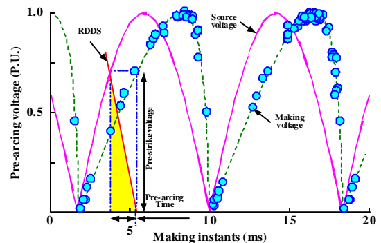
Fig.3 Typical pre-strike voltage against closing instant
