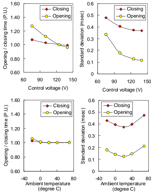
Fig.1 Variations of the closing and opening times from the average values at standard conditions and their deviations
