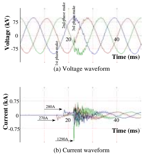
Fig.12 (a) Waveforms of the 1st capacitor energization
