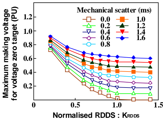
Fig.6 Dependence of maximum making voltage on RDDS and mechanical scatters in case of voltage zero targets
