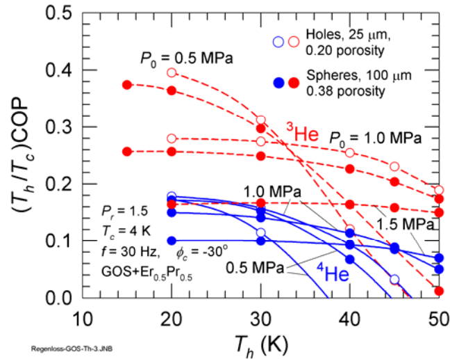
FIGURE 7. Effect of hot temperature and average pressure on regenerator second-law efficiency.
