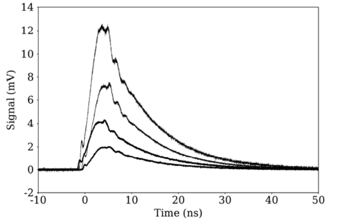
Fig. 2. Non-averaged signal voltage vs time for the four different parallel SNSPDs. Traces are in order bottom to top from the SNSPDs with four, eight, twelve, and twenty-four parallel nanowires all using an in series inductance of 470 \text{ nH} . The bias currents were 39 \mu\text{A} , 80 \mu\text{A} , 140 \mu\text{A} and 255 \mu\text{A} respectively. The temperature was 5 K.
