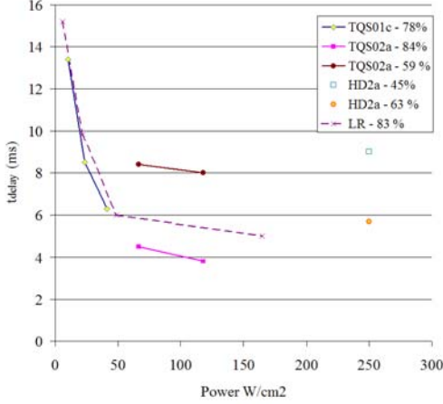
Fig. 4. Delay time in ms versus Heat deposition in \text{W/cm}^2 for several Nb3Sn magnets. The percentage corresponds to the short sample current fraction at which the data are given.
