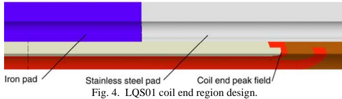
Fig. 4. LQS01 coil end region design.
