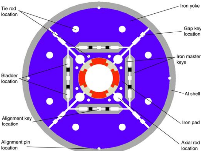
Fig. 2. LQS01 cross-section.
