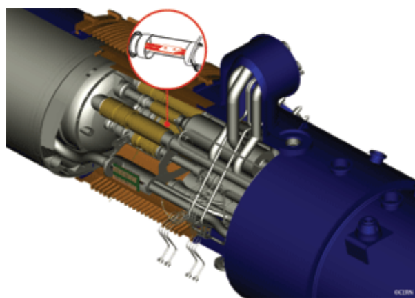
Fig. 1. Investigations have shown that a faulty electrical connection between two magnets (shown in red) was the cause of the incident in sector 3-4 of the LHC on 19 September, 2008.
