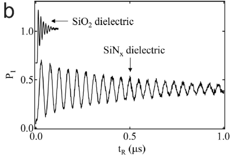
Fig. 1. (a) Micrograph of Josephson phase qubit circuit. (b) Rabi oscillations for phase qubit circuits incorporating PECVD-grown SiO 2 and SiN x wiring dielectrics. The factor 20 improvement in loss tangent for the SiN x compared to the SiO 2 yields a factor 20 enhancement in qubit energy relaxation time. Reprinted figure with permission from [5]. Copyright 2005 by the American Physical Society.
