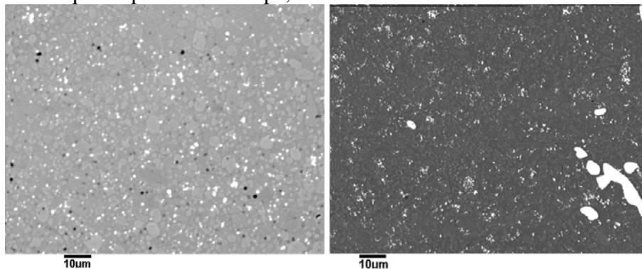
FIGURE 2. Electron microprobe images of textured YBCO superconductors. The sample on the left is Y123 + 30 mol% Y211 + 0.84 mol% \text{WO}_3 . Profuse W-rich deposits are the small bright white spots. Y211 particles (pale gray in color) are embedded in a gray Y123 background. The sample on the right is Y123 + 30 mol% Y211 + 4.12 mol% Pt + 1.25 mol% \text{WO}_3 . (W + Pt)-rich deposits are profuse small bright white spots while Y211 deposits appear as pale black in color and the YBCO background is black in color.
