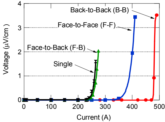
Fig. 4. Voltage-current characteristics of parallel-connected YBCO coated conductors.
