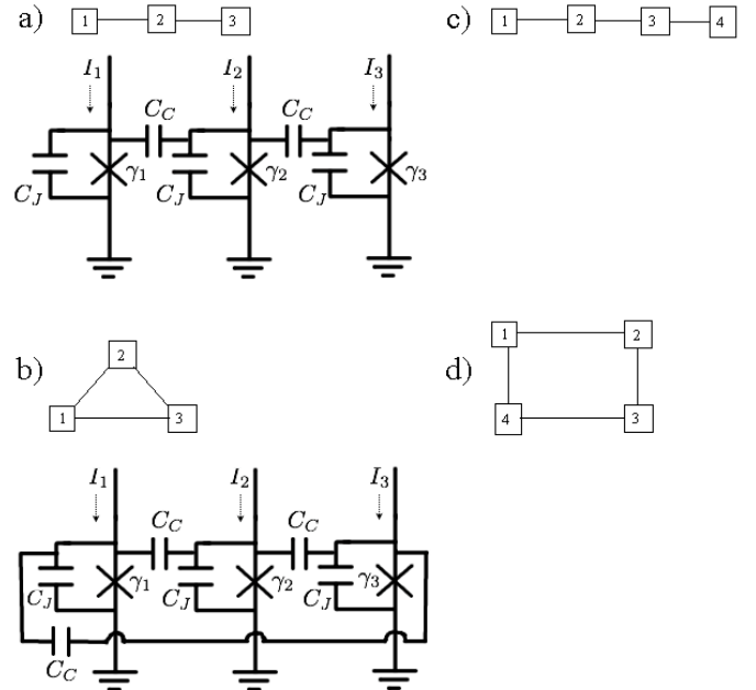
Fig. 1. (a) The linear three-qubit system and its corresponding circuit diagram. Each numbered square represents a junction and each line connecting them represents a coupling capacitor. (b) The triangular three-
