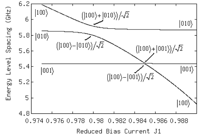
Fig. 2. Energy level spectrum for the linear three qubit system. Here J_2 = 0.979 , J_3 = 0.985 , while J_1 is being ramped. Qubits 1 and 2 become entangled when J_1 is slightly detuned from J_2 but far from J_3 . Qubits 1 and 3 become entangled when J_1 = J_3 . The energy gaps of the avoided crossings are different because qubits 1 and 3 have much weaker coupling than 1 and 2.
